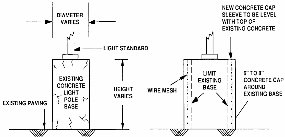
EXISTING BASE - DEFECTIVE CONCRETE
